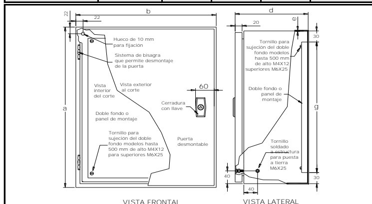
GABINETE TIE NEMA 12
